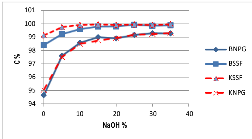
Figure 1. Effect of NaOH concentration on upgrading the carbon content in vein graphite
